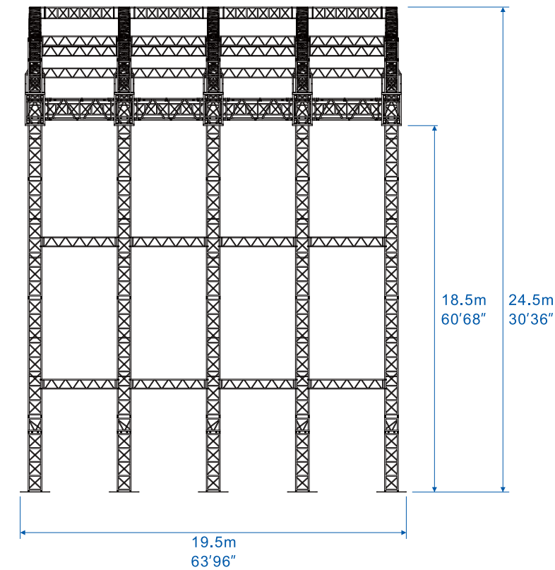
侧视图 Side view
